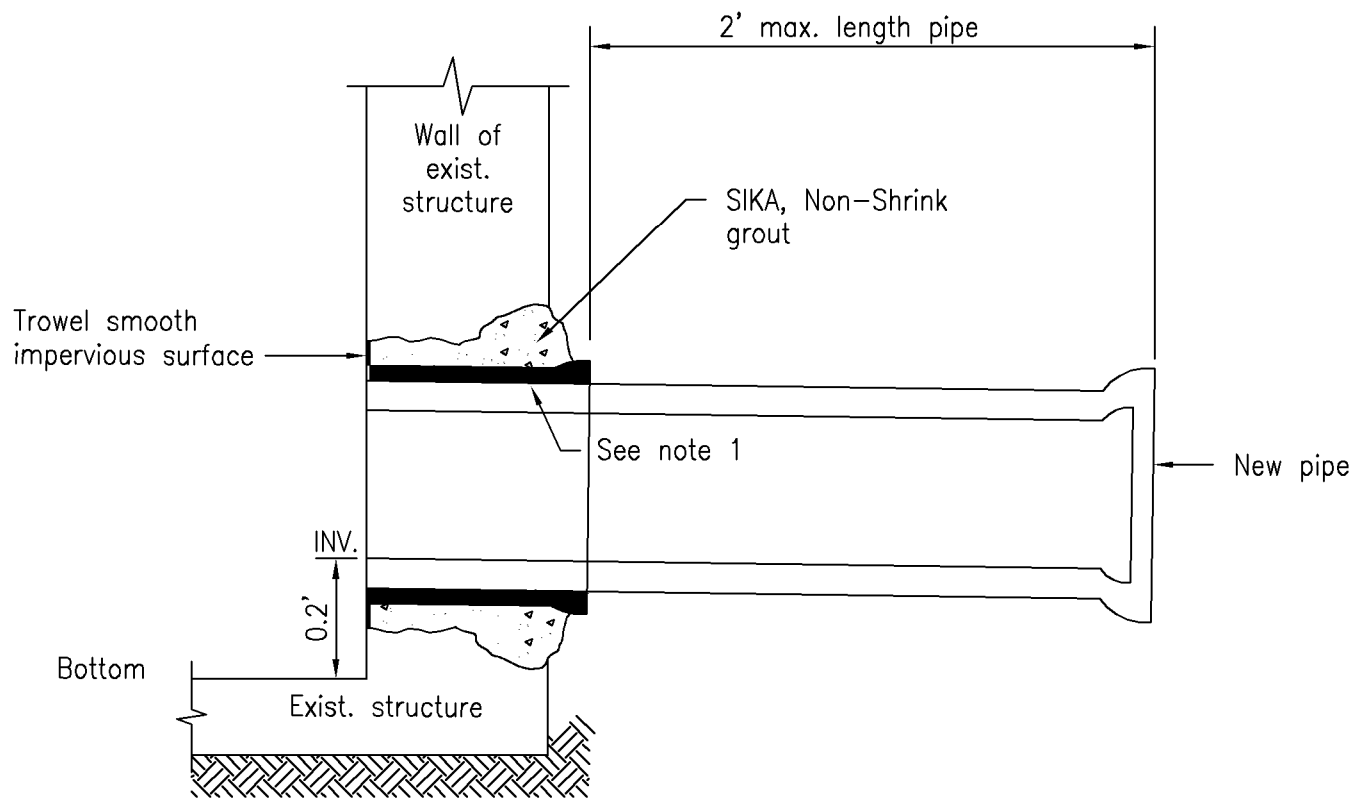
CONNECTION TO EXIST. STRUCTURE
